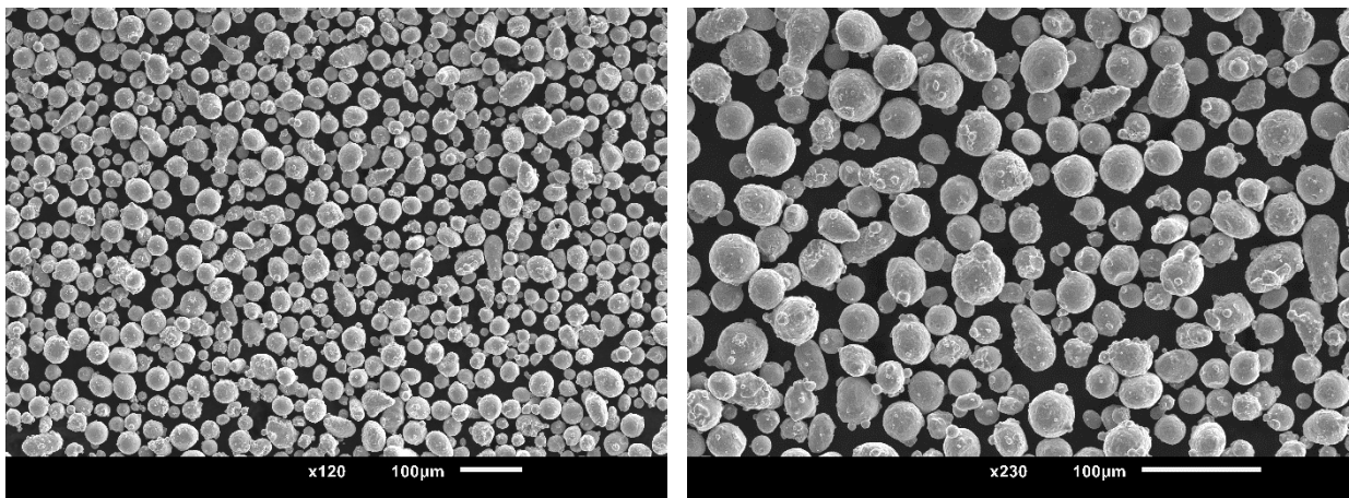
SEM micrographs of a) -45 +15 µm powder with a spherical morphology, b) smooth surface and low level of powder satellites
