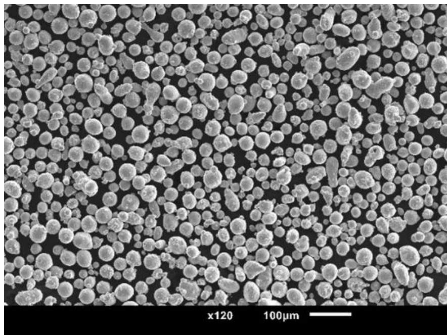
SEM micrograph of -45 +15 \mu\text{m} stainless steel powder with spherical morphology. Data source: University of Louisville.
