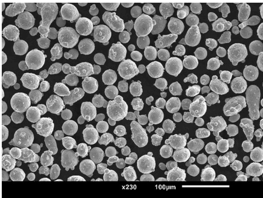
SEM micrograph showing smooth surface and low level of powder satellites. Data source: University of Louisville.
