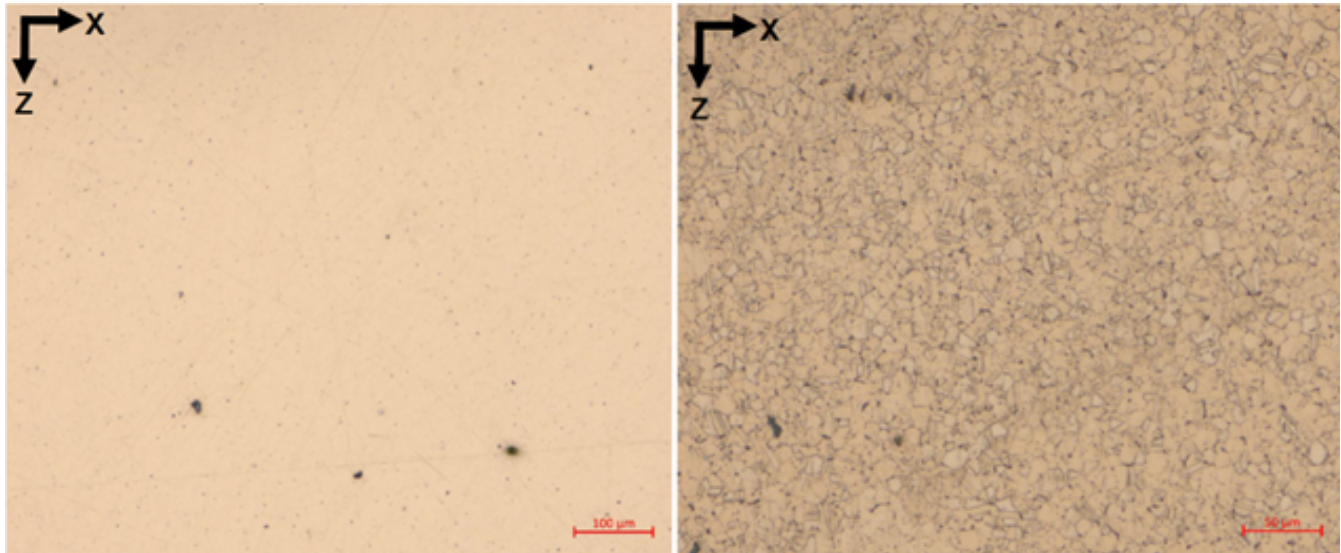
Micrograph of Osprey® C18150 in a) as-printed and b) etched conditions.
